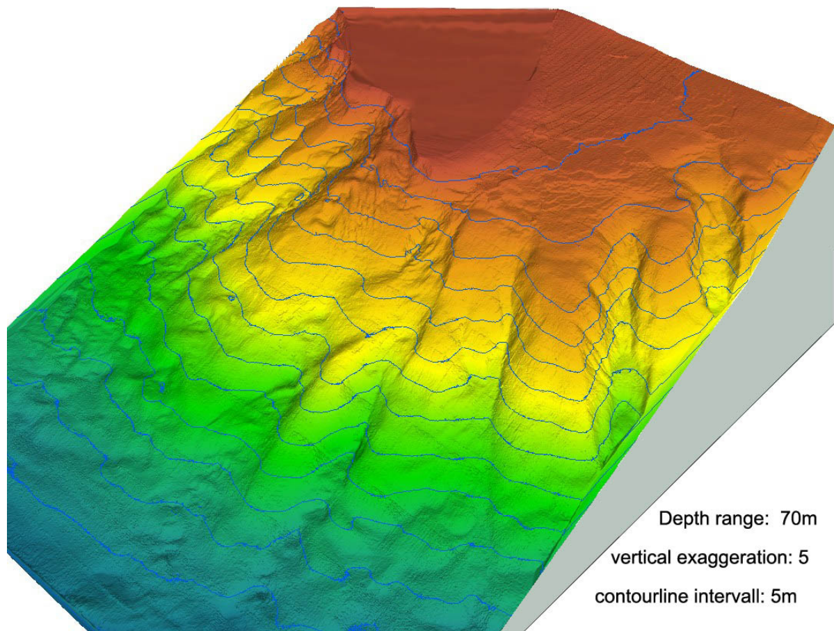
Figure 4: True-to-detail digital terrain model of the subaqueous delta plain of the Rhine created from multi-beam echosoundings
