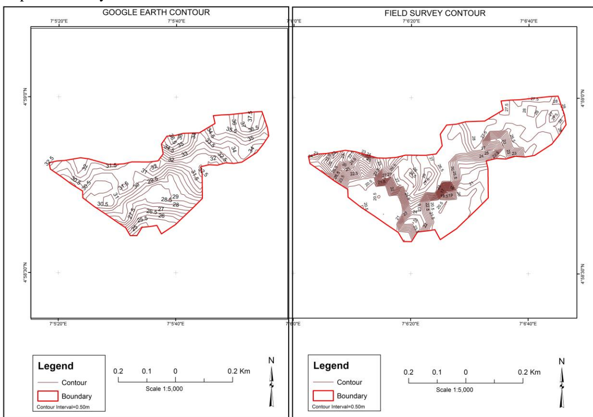
Figure 5. Contour surface from Google Earth. Figure 6. Contour surface from field survey.
