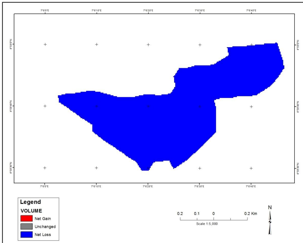
Figure 7. Cut and Fill volume from Google Earth and field survey.
