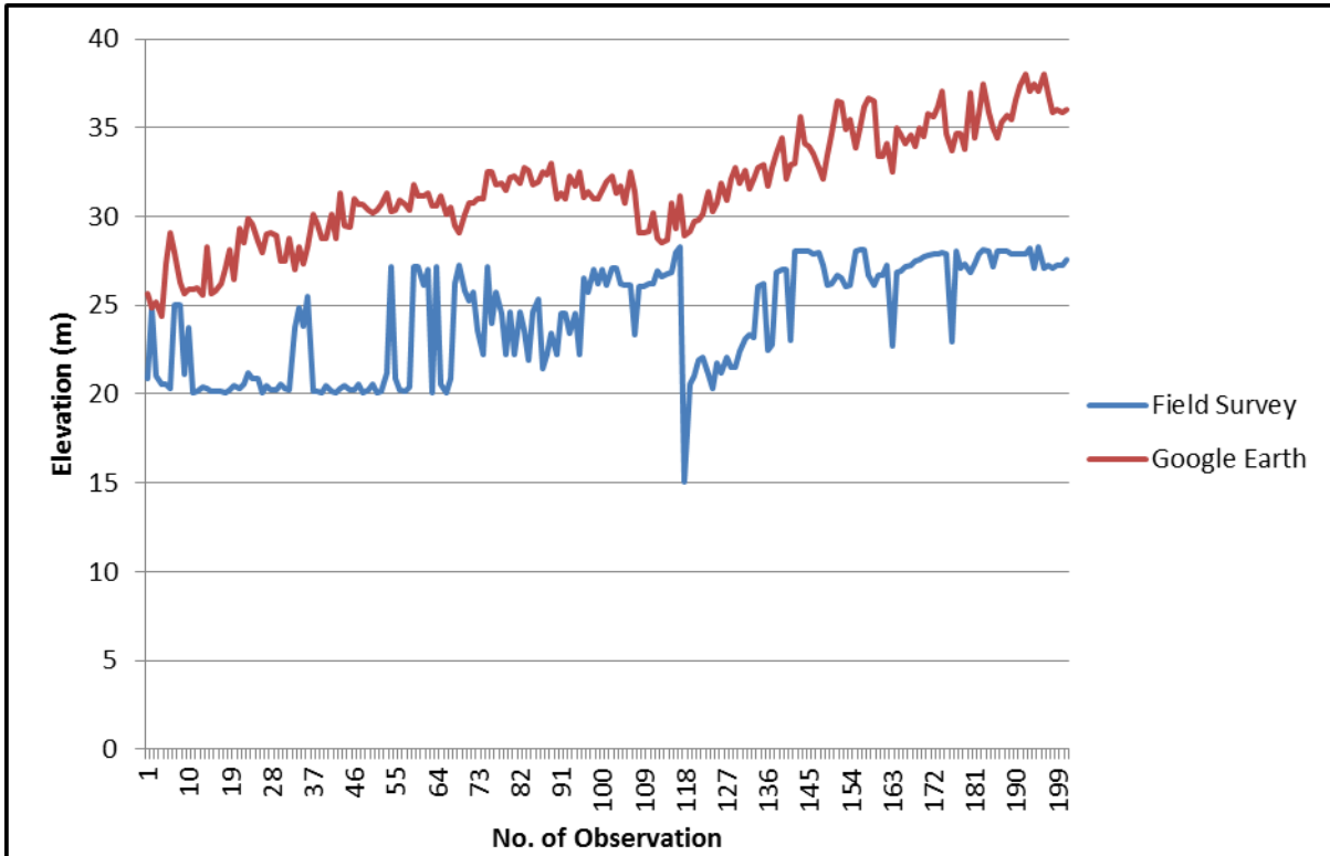
Figure 8. Scatter plot of field survey and Google Earth elevation data.
