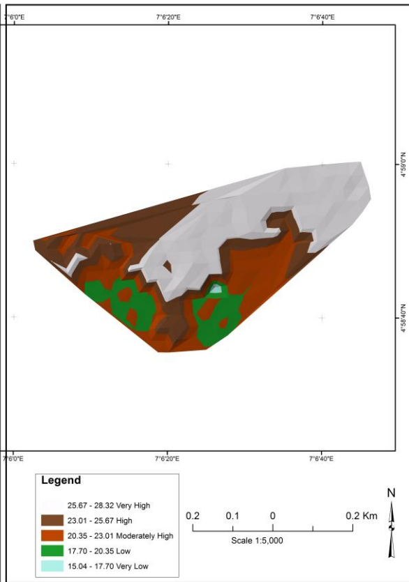
Figure 4. TIN DEM from field survey.
